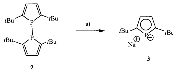
Scheme 2. Synthesis of \text{Na}(\text{Htp}) ( 3 ); reagents and conditions: a) excess Na, THF, room temp., 85%
