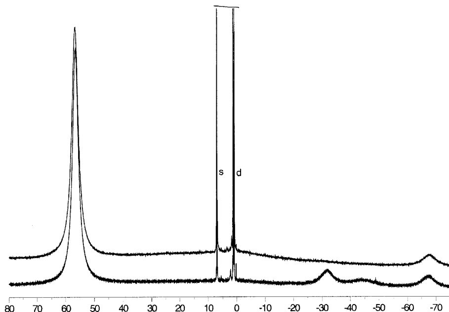
Figure 1. Proton NMR spectra (C 6 D 6 solutions, ppm values) of 10-d (upper trace) and 10 (lower trace) (s = C 6 D 5 H, d = diamagnetic impurities)
