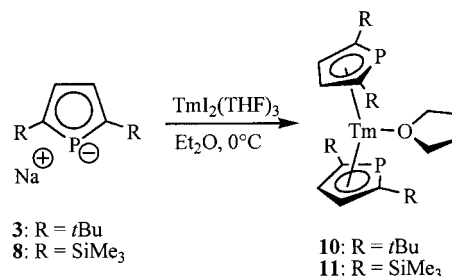
Scheme 4. Synthesis of Tm II phospholyl complexes
