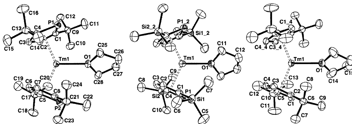
Figure 2. ORTEP plots of 10 , 11 and 12 together with the numbering schemes used (50% probability ellipsoids, H atoms omitted)
