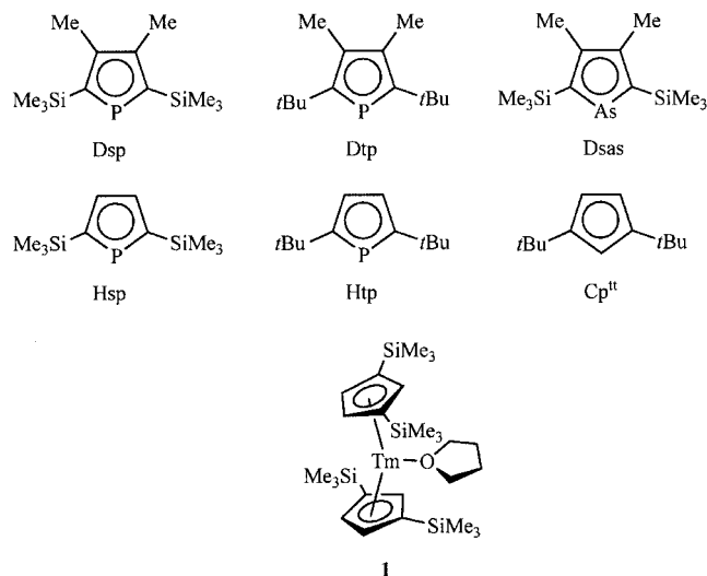
Scheme 1. Ligands and complexes in \text{Tm}^{\text{II}} chemistry
