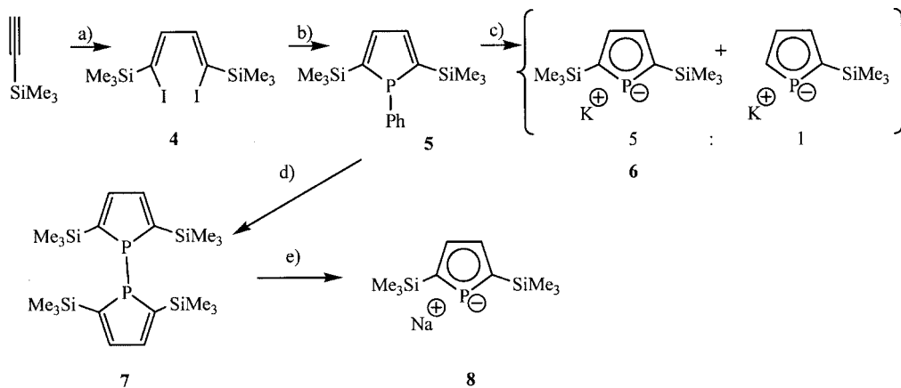
Scheme 3. Synthesis of \text{Na}(\text{Hsp}) ( 8 ); reagents and conditions: a) \text{Ti}(\text{OiPr})_4 + i\text{PrMgCl} , \text{Et}_2\text{O} , -78^\circ\text{C} to -50^\circ\text{C} , 2 h, then \text{I}_2 , -50^\circ\text{C} to room temp., 2 h, 67%; b) 2 n\text{BuLi} , \text{Et}_2\text{O} , -78^\circ\text{C} to room temp., 1 h, then \text{PhPCl}_2 , -78^\circ\text{C} to room temp., 30 min, 42%; c) excess K, DME, 70^\circ\text{C} , 2 h; d) excess Li, THF, room temp., 3 h, then \text{AlCl}_3 , 0^\circ\text{C} , 30 min, then \text{I}_2 , room temp., 15 min, 66%; e) excess Na, THF, room temp., 79%
