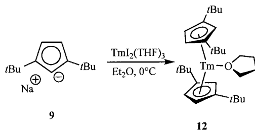
Scheme 5. Synthesis of a \text{Tm}^{\text{II}} cyclopentadienyl complex
